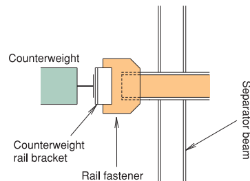
Example of fixing the counterweight rail brackets in A to a separator beam
