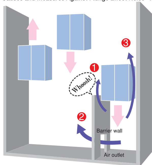
Figure 3. Causes and Measures Against Plunge Effect Noise -1
