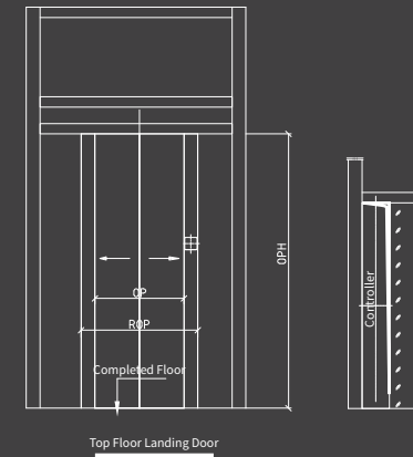
Top Floor Landing Door
