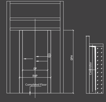
Top Floor Landing Door
