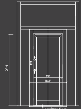
Top Floor Landing Door
