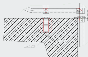
Variant A: Recessed bracket
